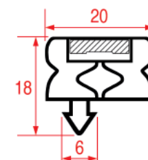
LF Profile: 1082 GEV Profile: 9251
