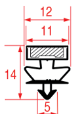
LF Profile: 1057 GEV Profile: 9020
