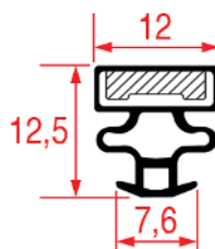
LF Profile: 1024 GEV Profile: 9373
